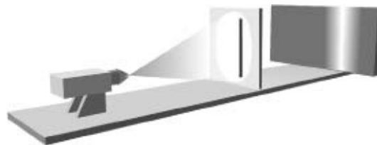
Figure 4.4 The right slit is open in this experiment, leading to an image on the photographic plate as shown.
