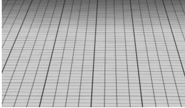
Figure 3.3 A schematic representation of flat space.
