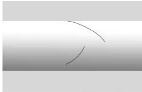
Figure 8.5 One Linebeing can see directly into the interior of another's body when Lineland expands into the Garden-hose universe.
