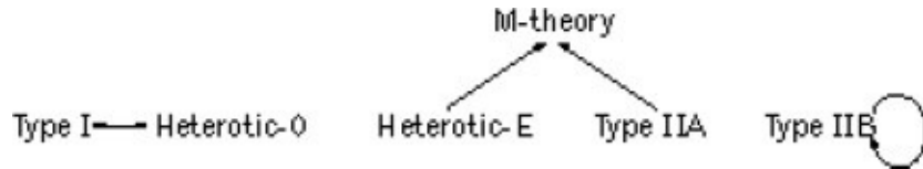
Figure 12.9 The arrows show which theories are dual to others.
