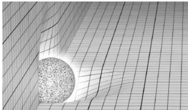
Figure 3.6 A sampling of the warped three-dimensional space surrounding the sun.
