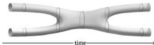
Figure 12.3 Strings interact by joining and splitting.
