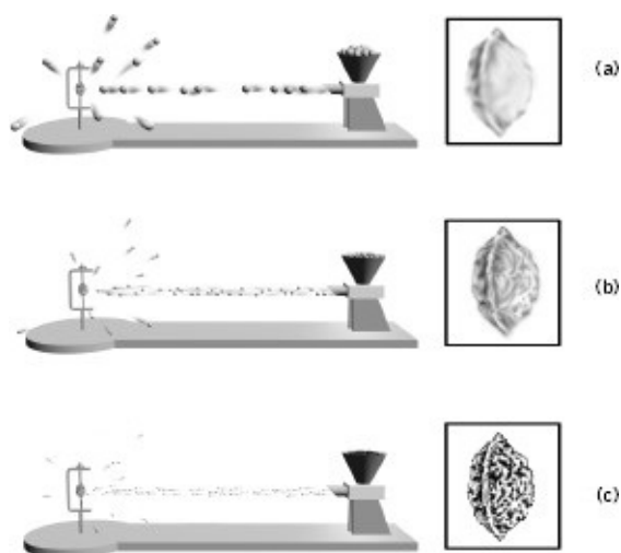
Figure 6.4 A peach pit is secured in a vise and it is drawn solely by observing how things—"probes"—thrown at it are deflected. By using ever smaller probes—(a) marbles, (b) five-millimeter pellets, (c) half-millimeter pellets—ever more detailed renditions can be drawn.
