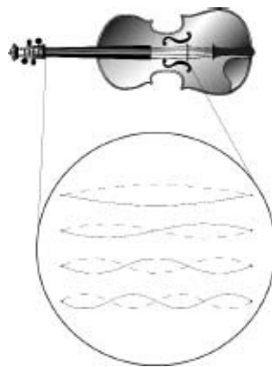
Figure 6.1 Strings on a violin can vibrate in resonant patterns in which a whole
