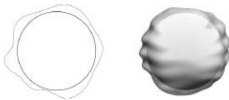
Figure 13.1 A string can encircle a one-dimensional curled-up piece of the spatial fabric; a two-dimensional membrane can wrap around a two-dimensional piece.
