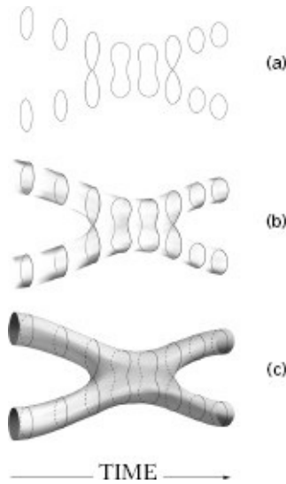
Figure 6.7 (a) Two strings on a collision course can merge into a third string, which subsequently can split apart into two strings travelling along deflected trajectories. (b) The same process as shown in (a), emphasizing string motion. (c) A "time-lapse photograph" of two interacting strings sweeping out a "world-sheet."
