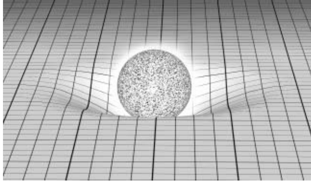
Figure 3.4 A massive body like the sun causes the fabric of space to warp, somewhat like the effect of a bowling ball placed on a rubber sheet.
