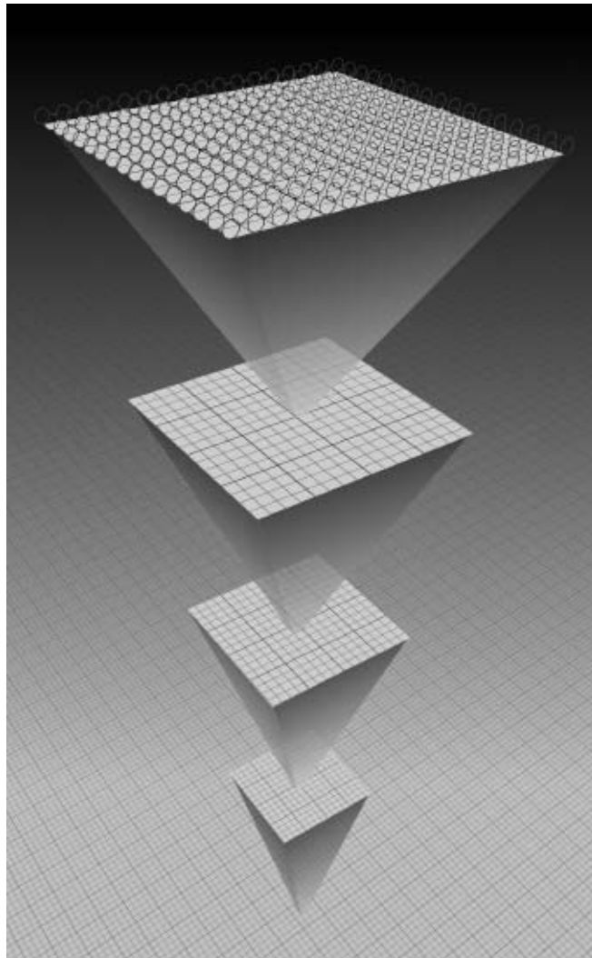
Figure 8.3 As in Figure 5.1, each subsequent level represents a huge
