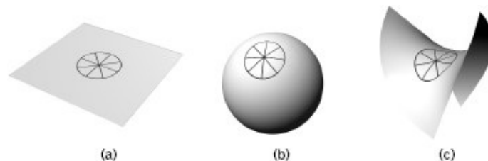
Figure 3.2 A circle drawn on a sphere (b) has a shorter circumference than one drawn on a flat sheet of paper (a), while a circle drawn on the surface of a saddle (c) has a longer circumference, even though they all have the same radius.
