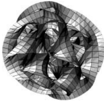
Figure 8.9 One example of a Calabi-Yau space.
